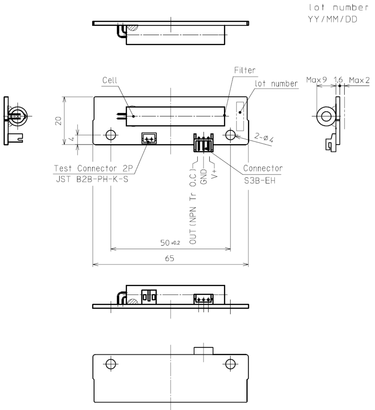
Figure 2: Dimensions
